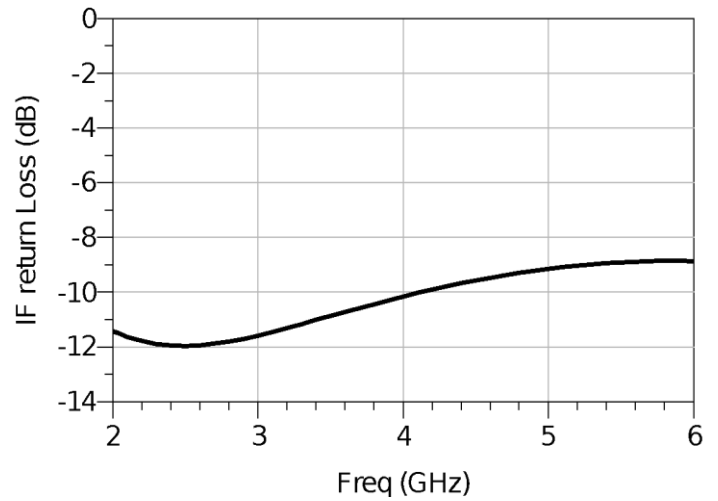
IF Port Return Loss
