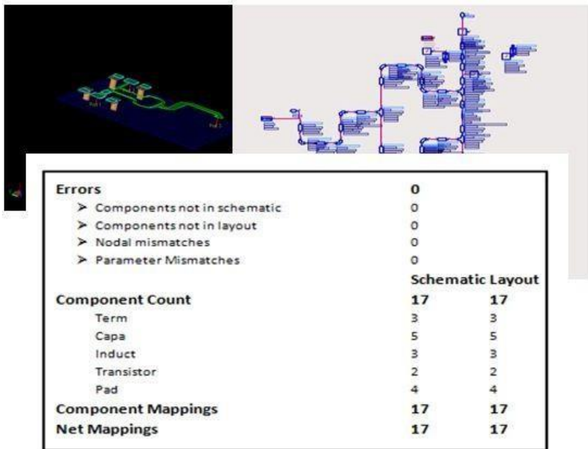
Figure 6: Layout Vs Schematic (LVS)
